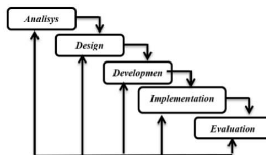
Gambar 1. Metode Waterfall
